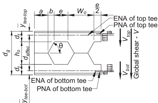
Castellated Beams
