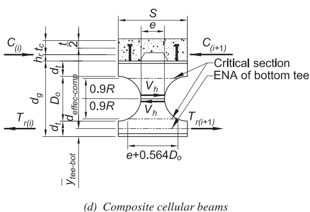
Fig. 3-6. Terminology used for calculating web post buckling.
