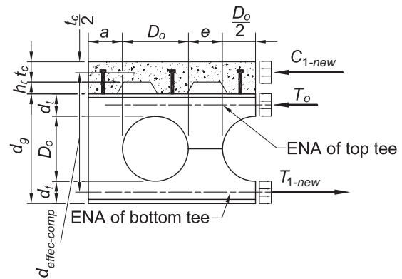
Cellular Beams
