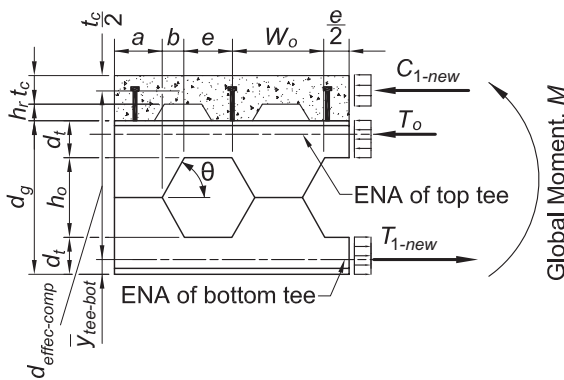
Castellated Beams
