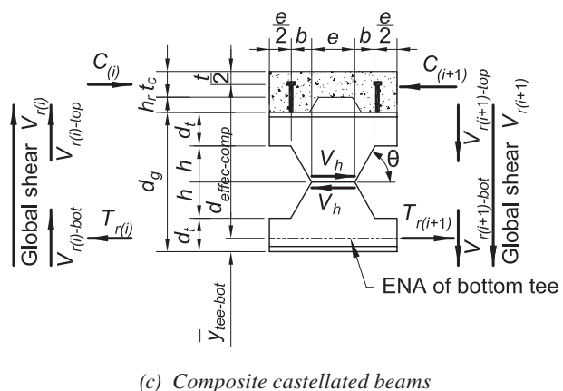
Fig. 3-6. Terminology used for calculating web post buckling.
