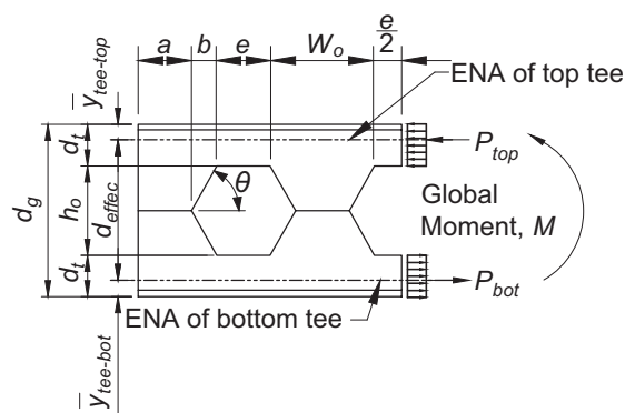
Castellated beam
