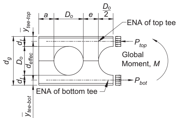
Cellular beam
